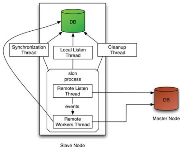
Figure 1. How the Slony-I replication engines work for a master with a slave database.
