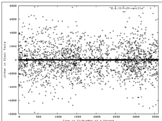
Figure 2. Jitter Results on a Vanilla 2.6.11-rc3 Kernel
