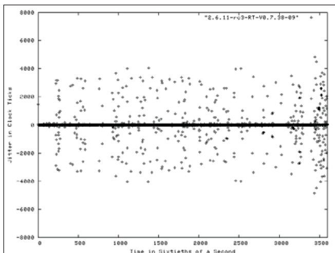
Figure 3. Jitter Results on a 2.6.11-rc3 Kernel with Real-Time/Preemption Patches
