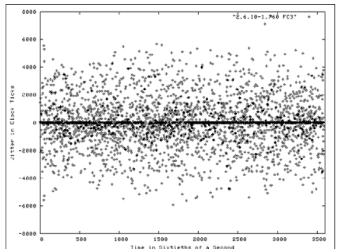
Figure 1. Jitter Results on a Stock Fedora Core Kernel
