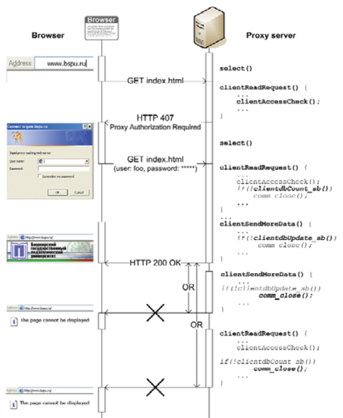
Figure 2. Simple Client Request Processing Diagram
