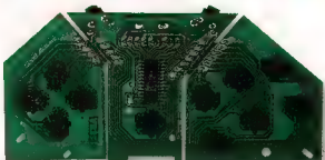
The curved boomerang shape of the U.S. Saturn controller necessitates a three-part integrated circuit board (above). The Japanese controller (below) reveals a far cleaner design, requiring half as many soldering points. The top button switches appear identical in both versions.
