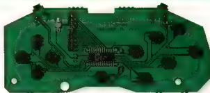
The curved boomerang shape of the U.S. Saturn controller necessitates a three-part integrated circuit board (above). The Japanese controller (below) reveals a far cleaner design, requiring half as many soldering points. The top button switches appear identical in both versions.
