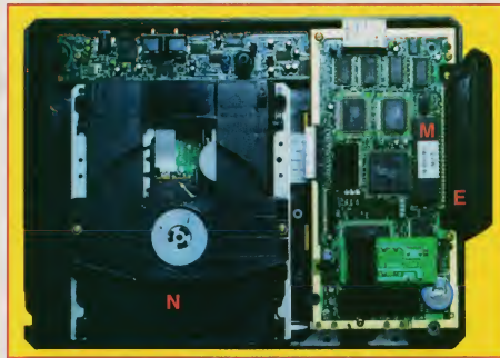
Inside the Mega CD-ROM
