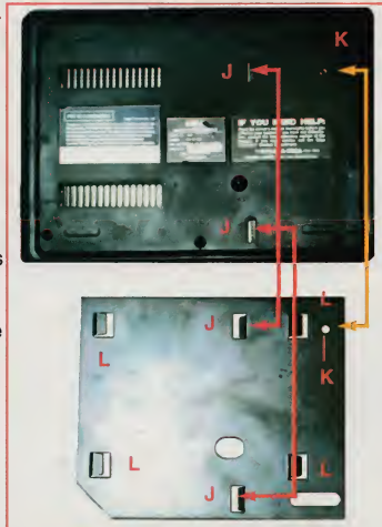
The metal plate provided with the Mega CD-ROM has to be slipped into the notches on the Genesis (red), and then securely fastened with the screw (orange).
