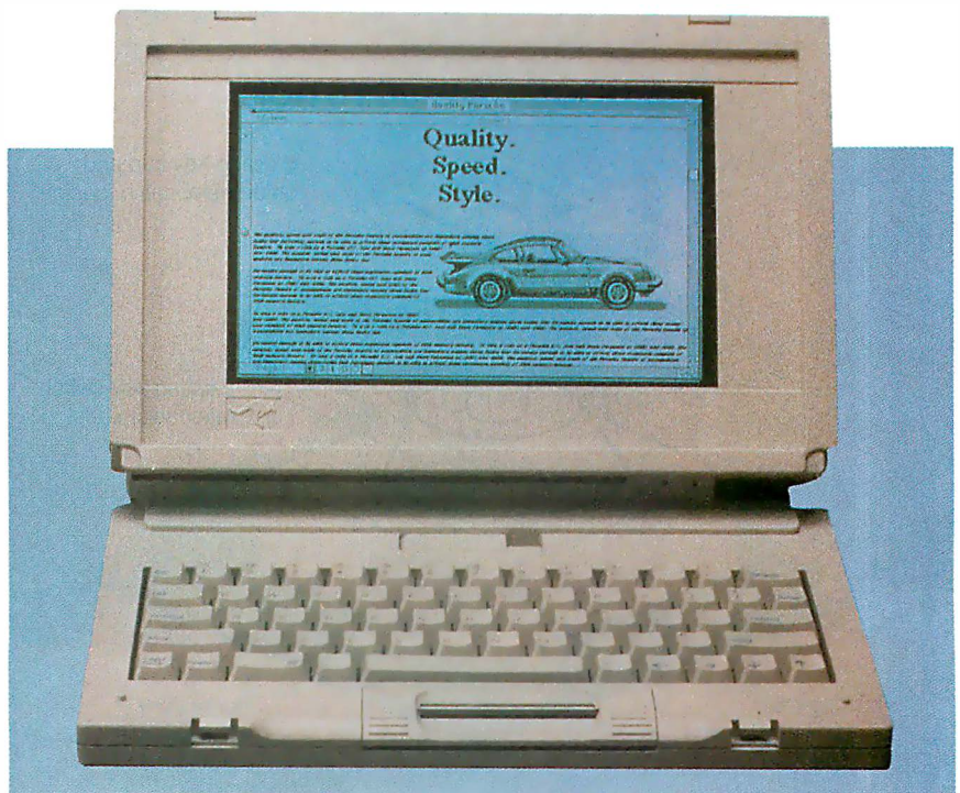
Photo 4: The Outbound Systems Macintosh-compatible laptop sacrificed the Mac Portable's cutting-edge display and trackball in favor of a normal LCD and the first use of the Isopoint pointer. Outbound's Isopoint is 4½ inches long and 1 inch high, and it resolves 101.6 pulses per inch of travel. Its low power usage keeps overall power consumption to a minimum.
