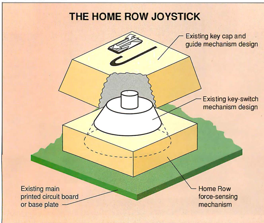
This pointer-in-a-keyboard uses no real estate and costs nearly nothing. The Home Row is a joystick embedded in the J key; when another key is toggled, the J key rocks on its base, moving the screen cursor. Key Tronic is manufacturing OEM keyboards with this feature under the name "KeyMouse."
