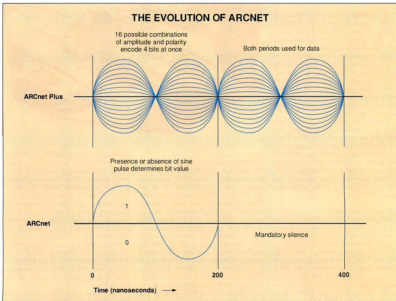
The original 2.5-Mbps ARCnet signals bit values by determining the presense or absence of a sine pulse. Here, ARCnet signals a "1" bit by sending a 200-ns pulse, followed by a silence of equal length. The 20-Mbps ARCnet Plus specification makes more efficient use of the bandwidth by using both periods for data and by using amplitude modulation to encode 4 bits into every pulse. ARCnet Plus also sends a calibration pattern once for every 8 bytes, further reducing overhead.
