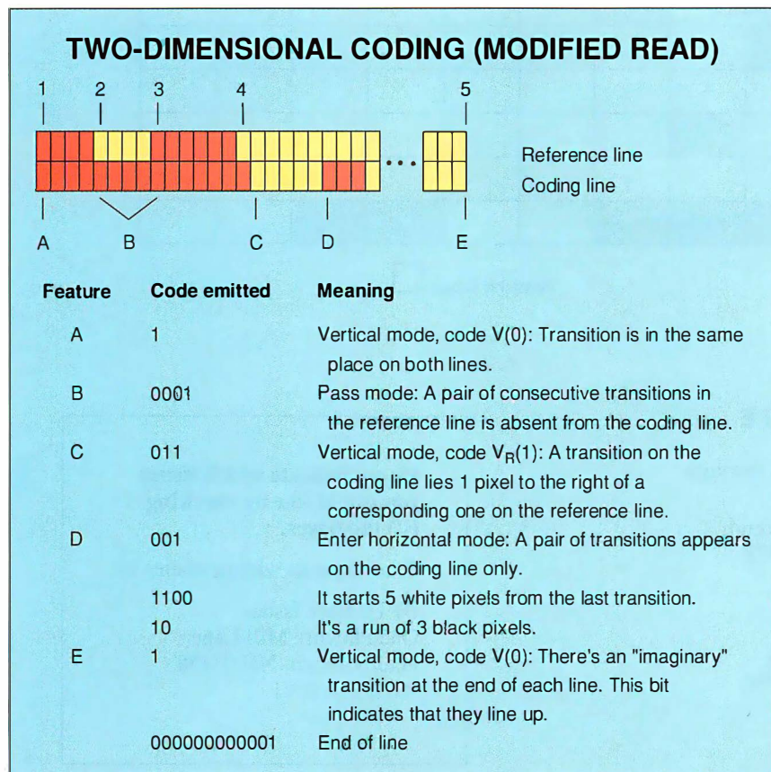
Figure 4: In two-dimensional coding ( modified READ , or relative addressing ), the sender looks for correspondences between the pixels on an earlier line (called the reference line ) and the current one (the coding line ). In vertical mode, the sender indicates that a transition is shifted up to 3 pixels left or right from one on the reference line. (This scheme is excellent for coding slanted lines.) In pass mode, the sender indicates that a pair of transitions on the reference line doesn't occur on the coding line and must be "passed by." Finally, in horizontal mode, the sender can indicate that there's a new pair of transitions on the coding line that wasn't there on the reference line.
