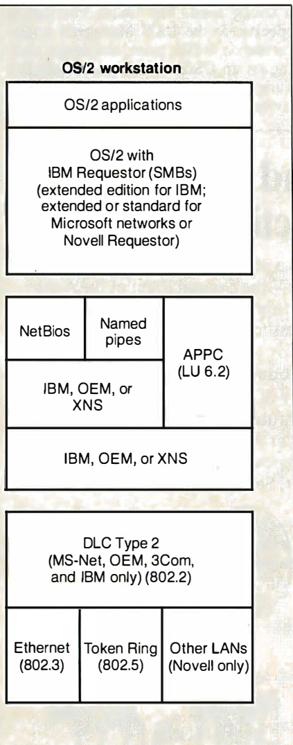
Figure 2: The Banyan VINES and OS/2 workstation architectures.
