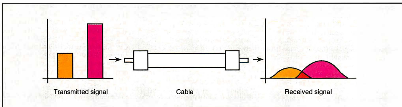
Figure 3: The change in signal levels over metallic cable. Beginning as a square wave, the typical digital signal will weaken and round off as it travels down the cable. As adjacent square waves do the same, the different pulses run into one another.
