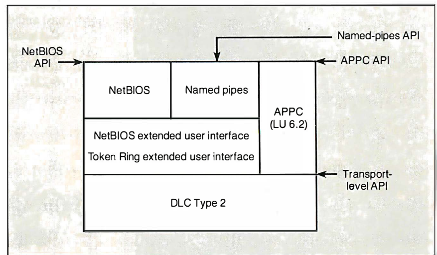
Figure 3: The APPC, NetBIOS, and transport-level APIs.
