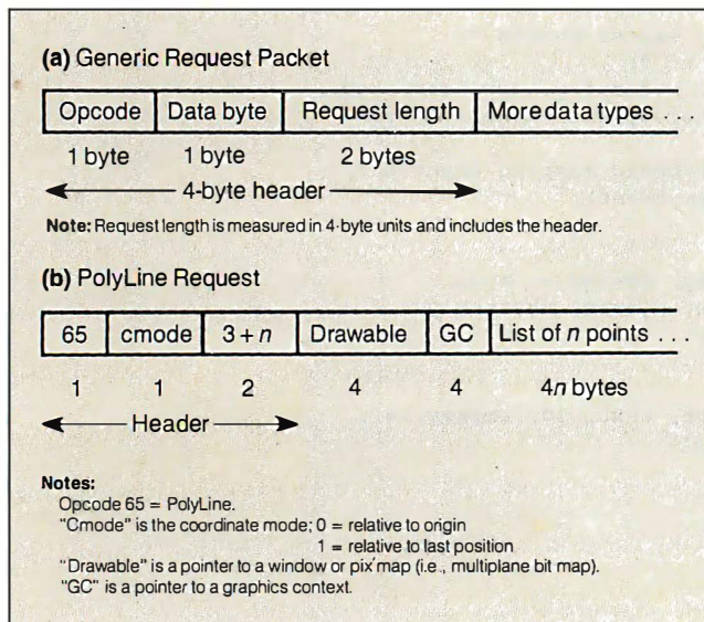
Figure 3: X Protocol request packets contain a 4-byte header and as many additional bytes as needed to communicate the request. The PolyLine request contains the information to draw a series of lines with a given line style and thickness within the graphics context.
