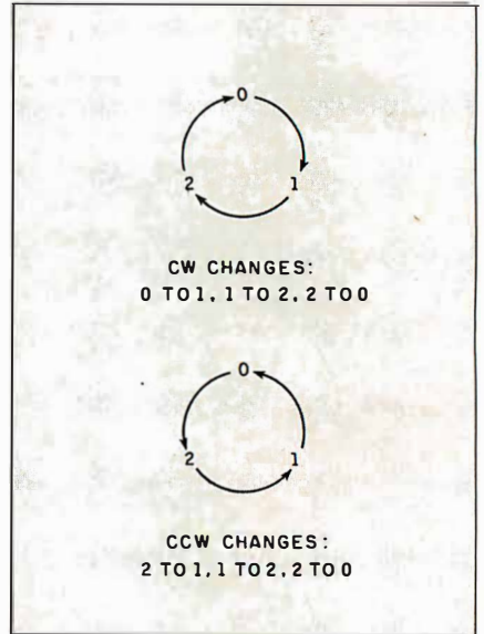
Figure 2: Illustration of clockwise and counterclockwise digit changes, for use in classifying numbers. A number is clockwise if its first digit change (starting at the left) is clockwise; otherwise, it is counterclockwise.
