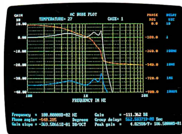
AC Analysis
