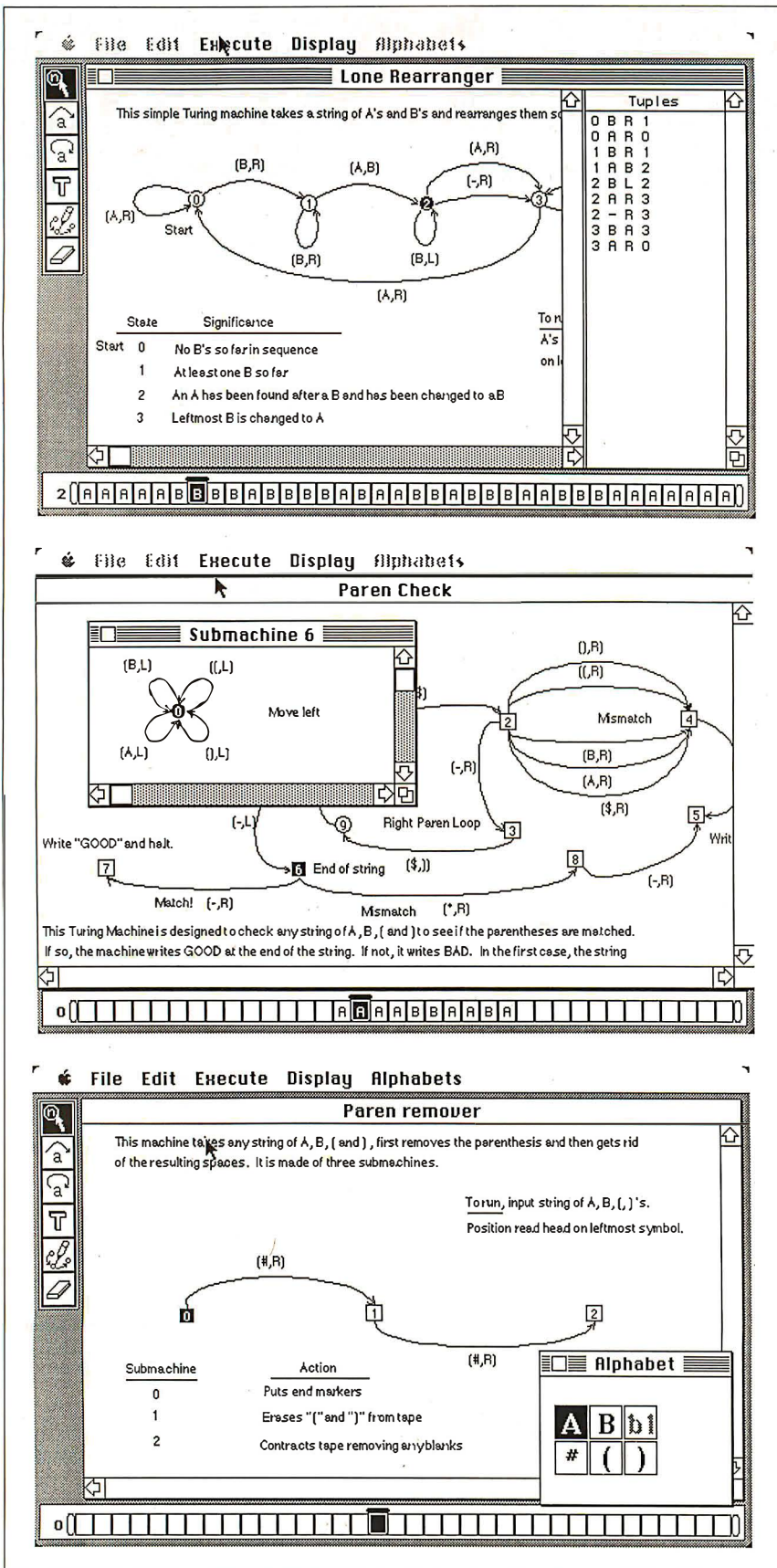
Figure 4: Turing's World by Jon Barwise and John Etchemendy of Stanford gives users a graphical environment in which to build, debug, and run Turing machines.
