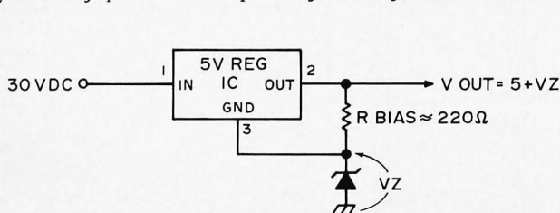
Fig. 6. Voltage pedestal technique using a 5 V regulator IC.
