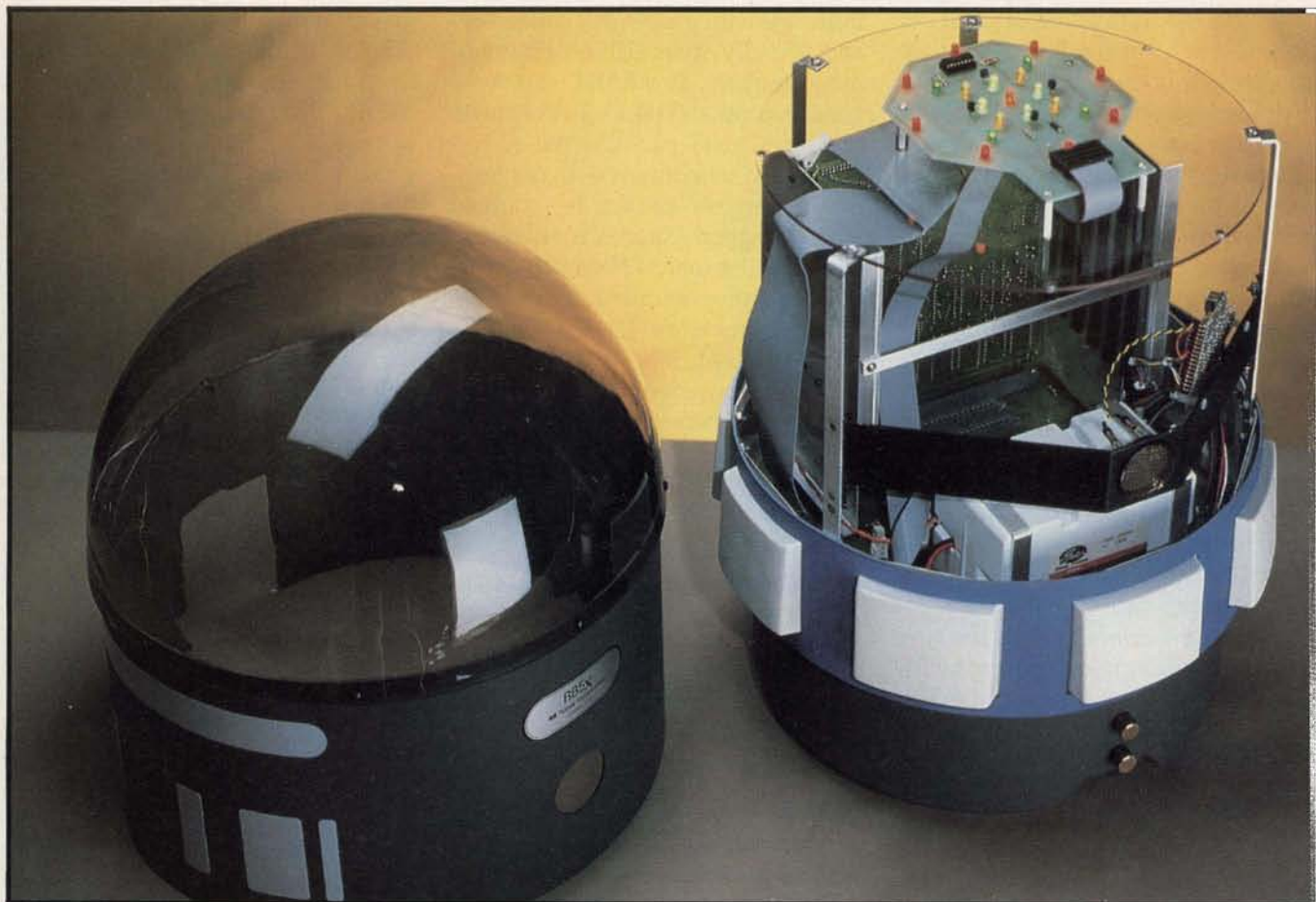
Photo 2: An internal view of RB5X that shows the main circuit board and rechargeable batteries.
