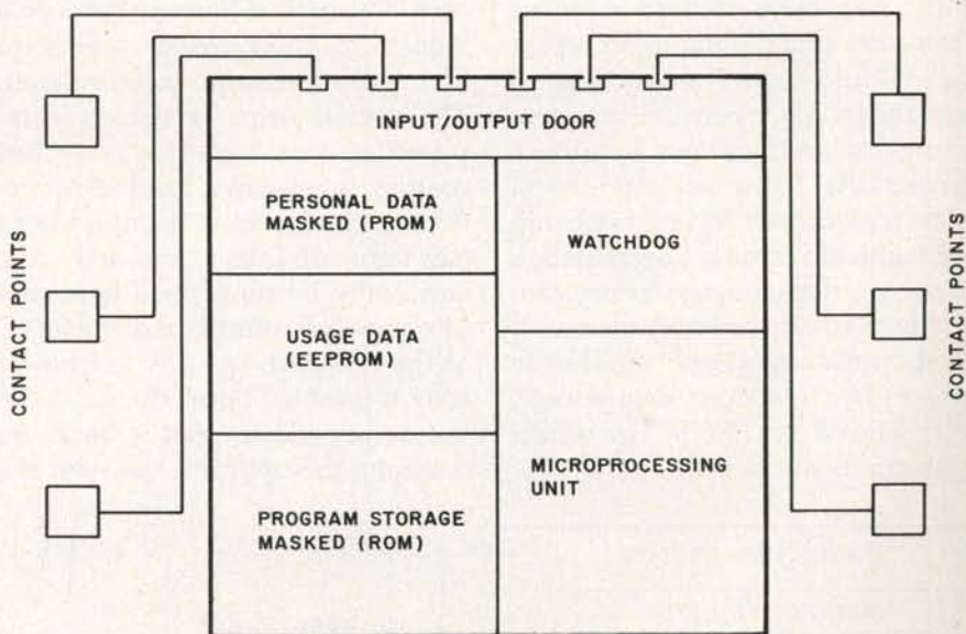
Figure 2: The system architecture of a monochip-based memory card.
