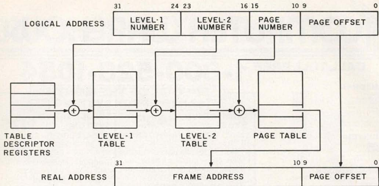
Figure 5: The Z80000 address translation scheme.
