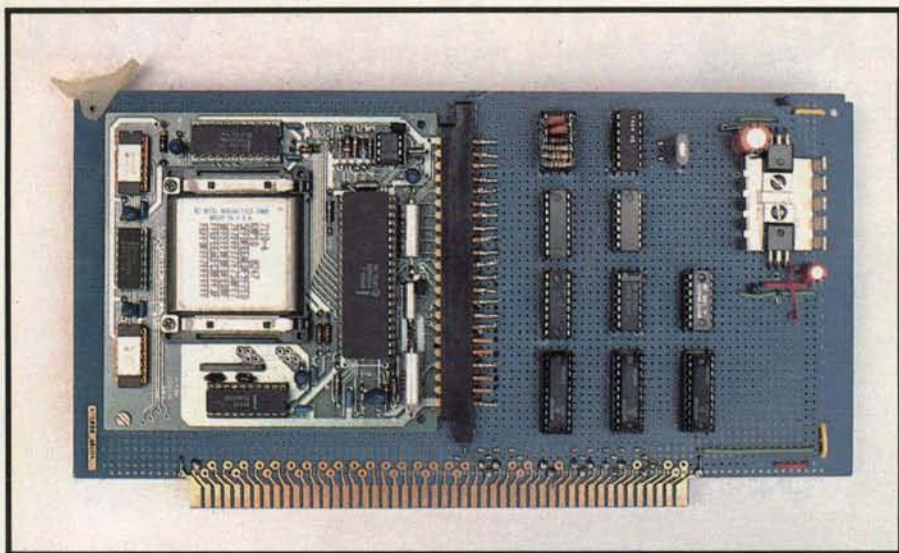
Photo 3: The completed S-100 bubble-memory board's component side with the BPK 72 installed (see figure 4 for the parts layout).
