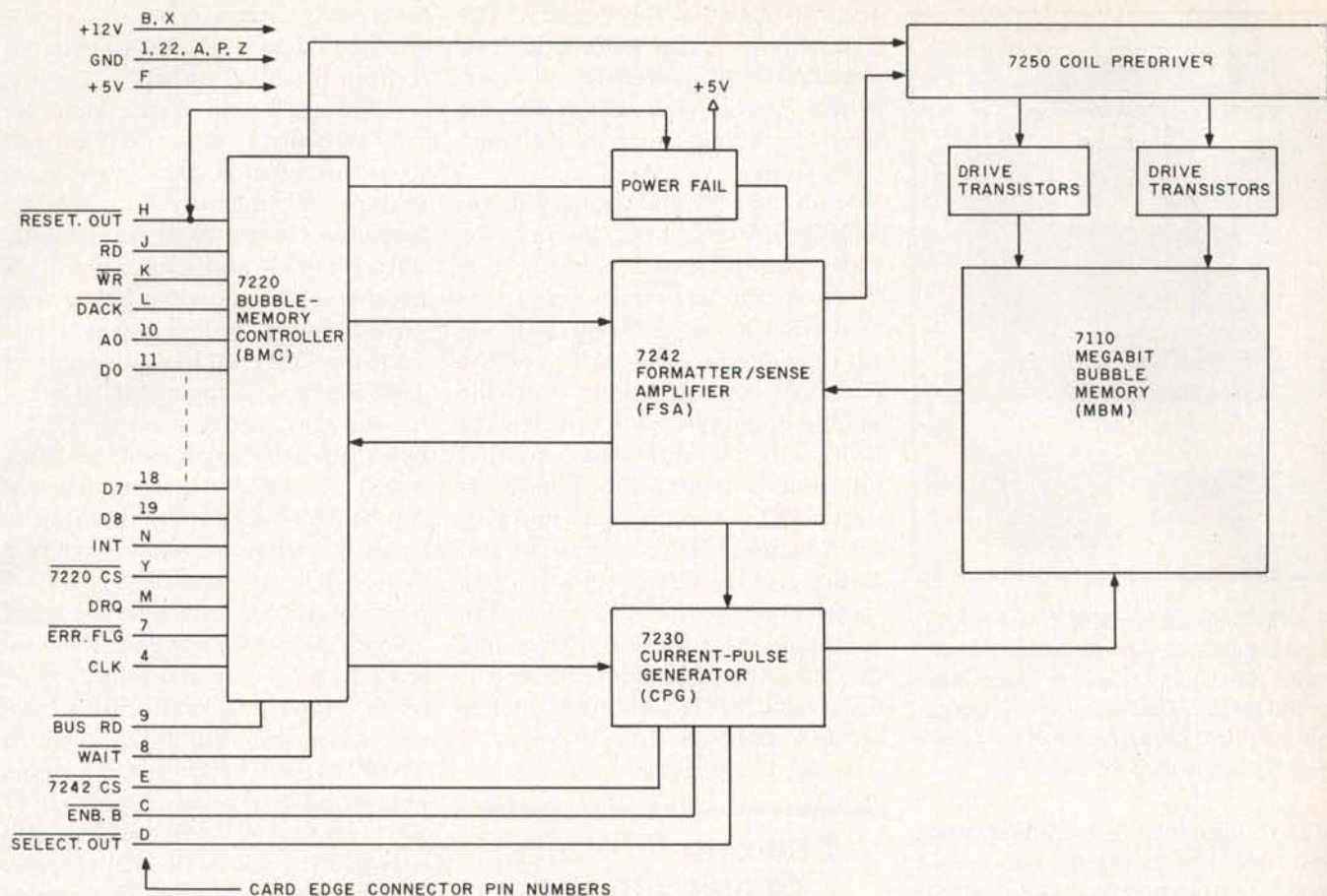
Figure 1: A block diagram of the BPK 72 Bubble-Memory Prototype Kit.
