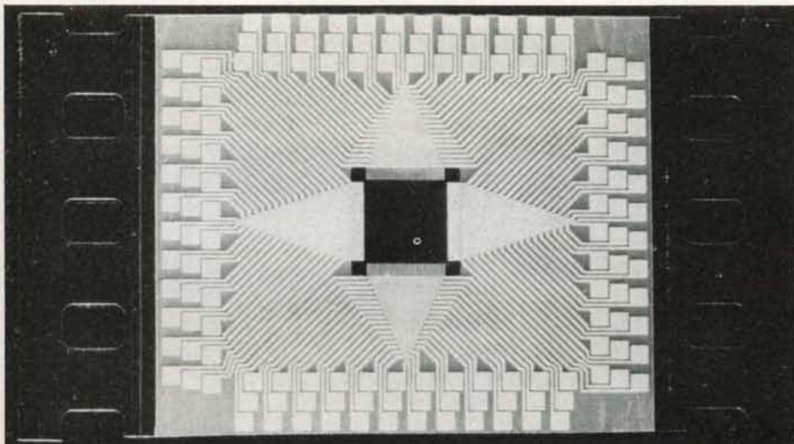
Photo 3: An integrated circuit bonded to a carrier tape or TAB (tape-automated bonding). This process is used to fabricate thin electronic devices such as calculators and memory cards.
