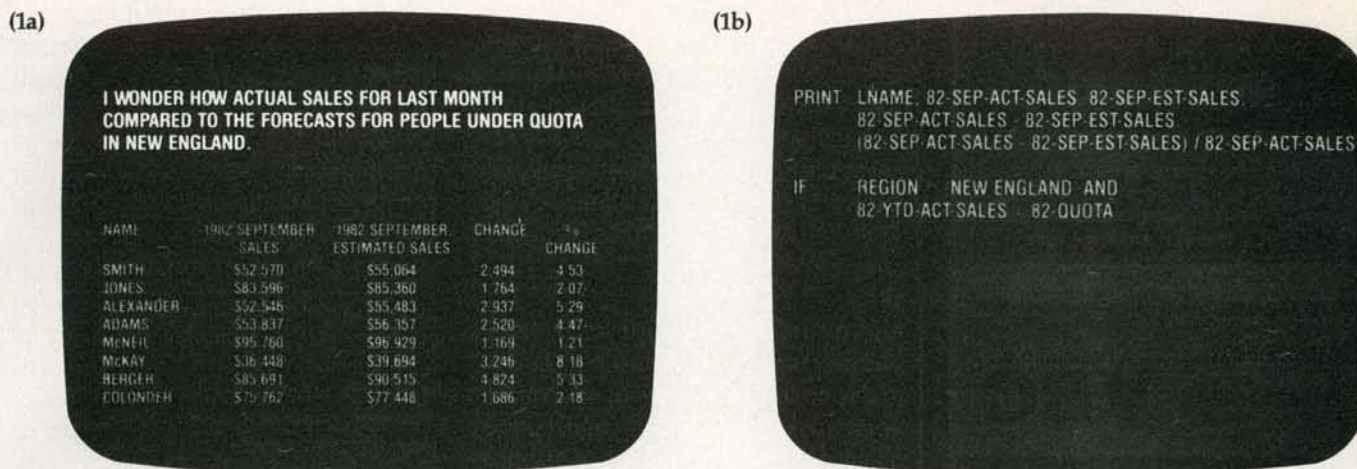
Figure 1: A comparison of English (a) and "English-like" (b) queries.
