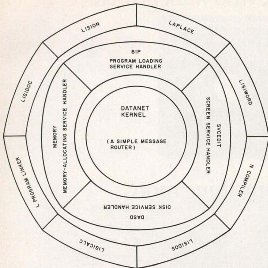
Figure 3: The Datanet system is constructed from a layered collection of discrete components with a single message router at the center. There are no operating systems or applications programs, just a collection of components, each sending messages to all the other components.
