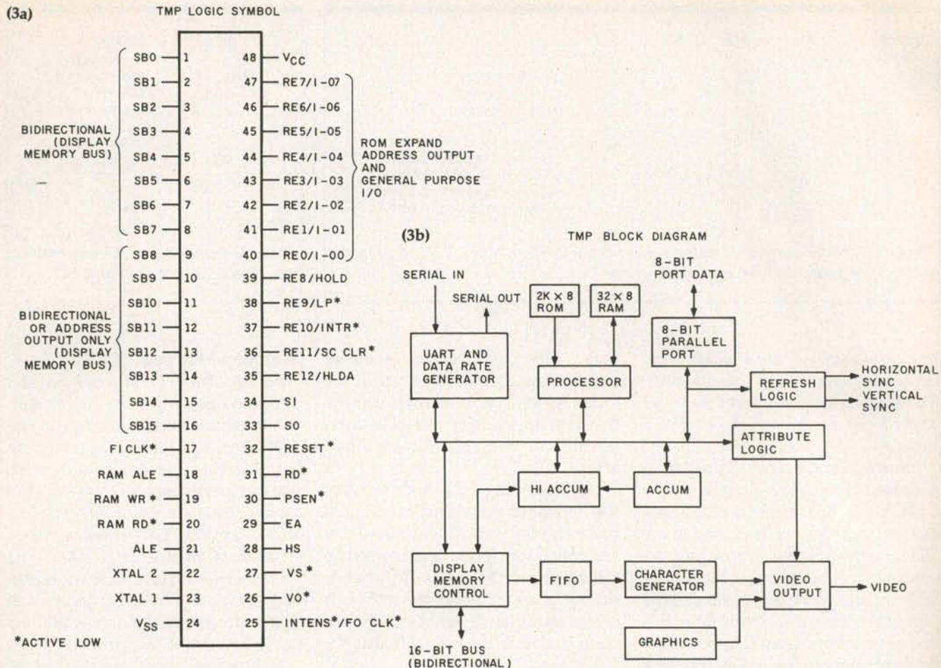
Figure 3: A pinout diagram (3a) and a block diagram (3b) of the National Semiconductor NS455A TMP.
