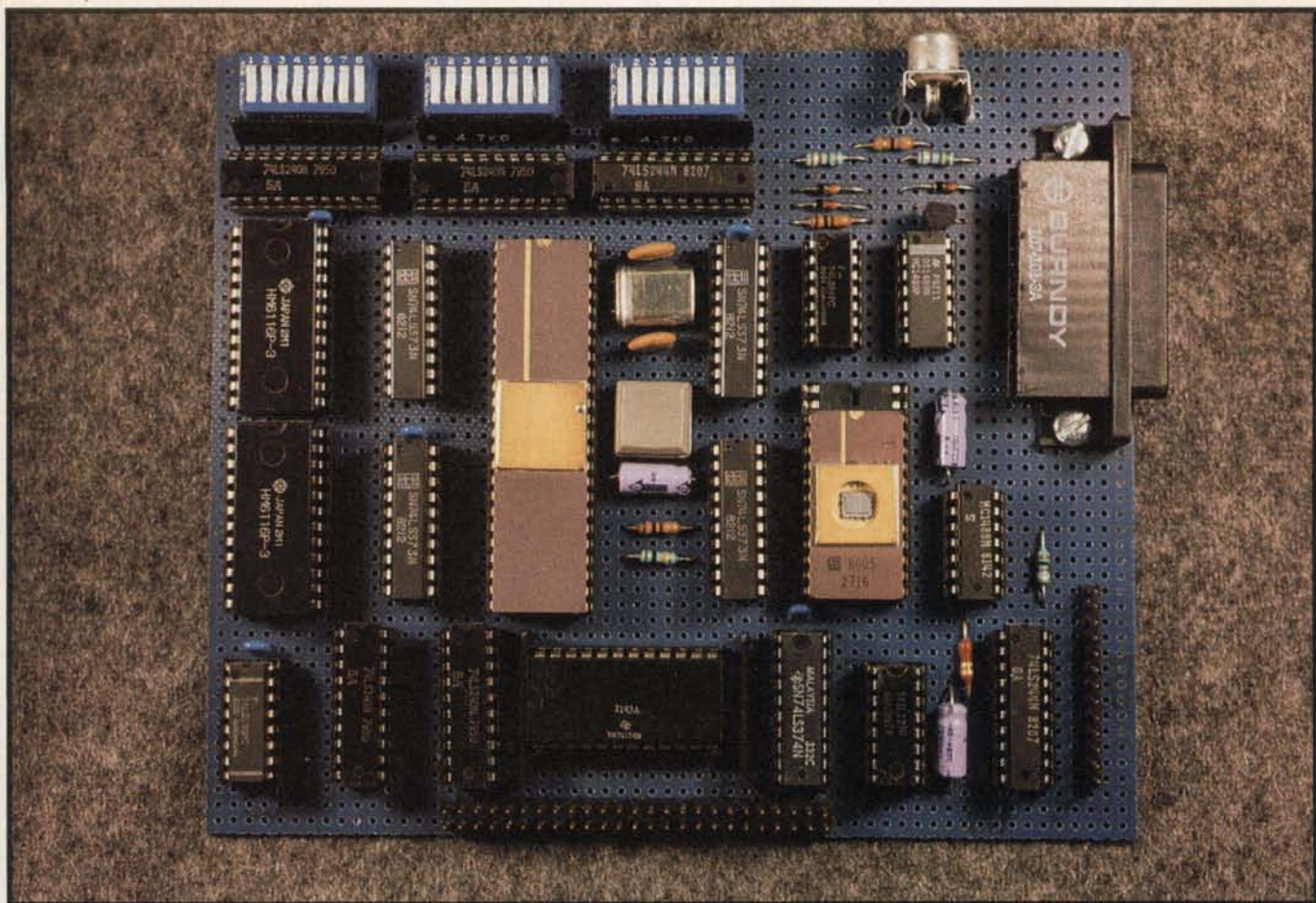
Photo 1: The prototype board of the Term-Mite ST intelligent video-display terminal.
