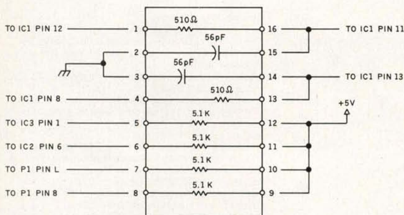
Figure 4: This top view of the DIP header wiring diagram includes all the resistors and capacitors (except power-supply bypass capacitors) shown in the figure 2 schematic. All resistors are 1/4 watt.
