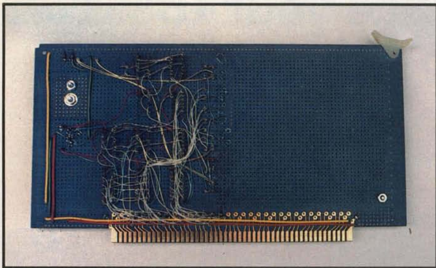
Photo 4: The wiring side of the S-100 bubble-memory board. The following color code applies: red = +5 volts, yellow = +12 volts, green = ground, and white = signal.
