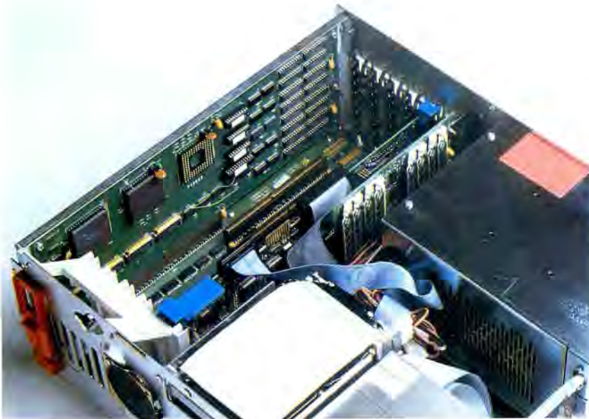
Photo 1: The CPU card is visible in the upper left corner. The card contains the 80386, a socket for an 80387 coprocessor, the 82385, and the SRAM cache chips.
