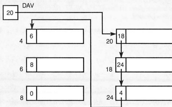
Figure 2: Once DELETE_KEY has removed the associated key, deleting an entire record set is simply a matter of attaching the set to the available-for-reuse list.
