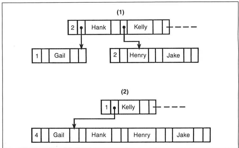
Figure A: A sample order-4 B-tree. (1) A key has been deleted, leaving Gail all alone on its node. (2) Merging Gail with the father key and right sibling reduces two near-empty nodes to a single full node. Of course, the node containing Kelly might now be merged with its sibling.
